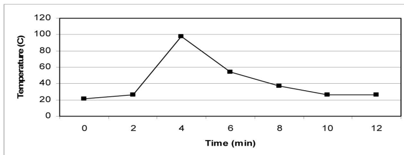
Typical Exotherm Curve for MA420FS at 23°C (10 grams) 5
