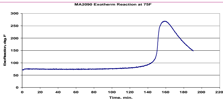
Typical Exotherm Curve for MA2090 at 23°C (30 grams) 5
